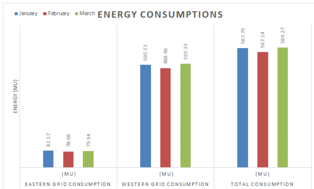
Graph 3.1.2. Energy (MU) consumed
