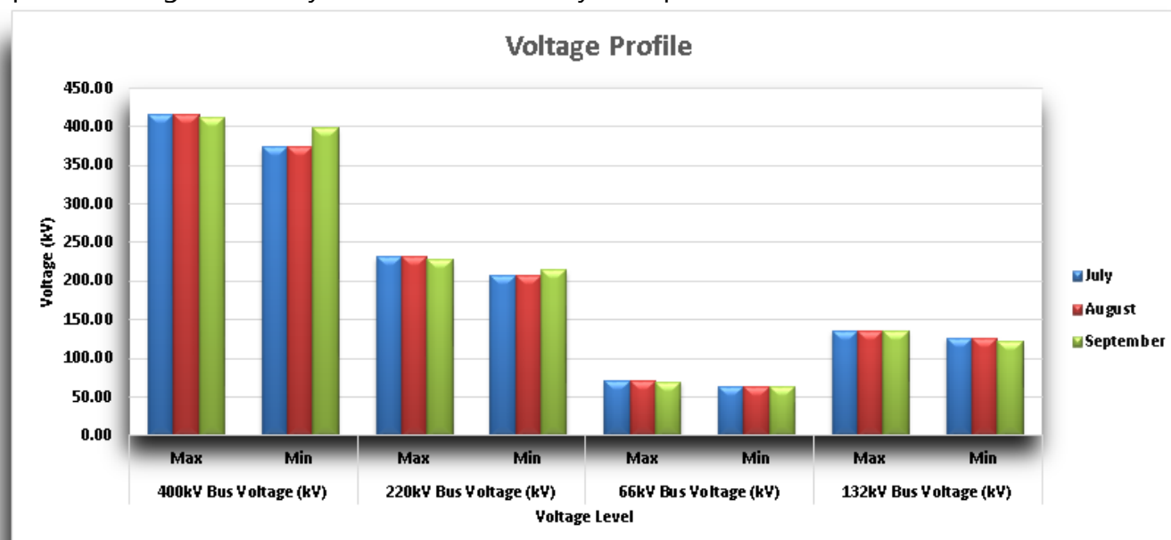
Graph 9.1 Voltage Summary for the month of July to September 2025
