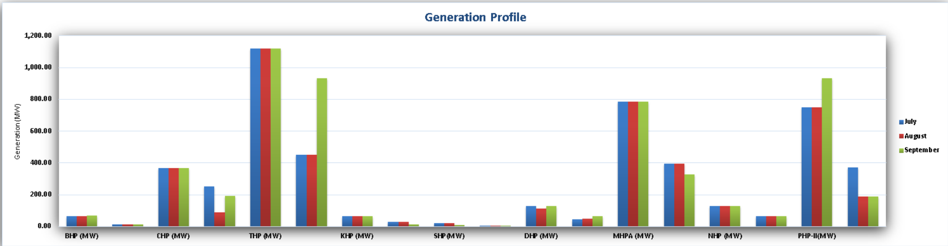
Graph: 6.1 Summary of maximum and minimum generation by various hydropower plants
